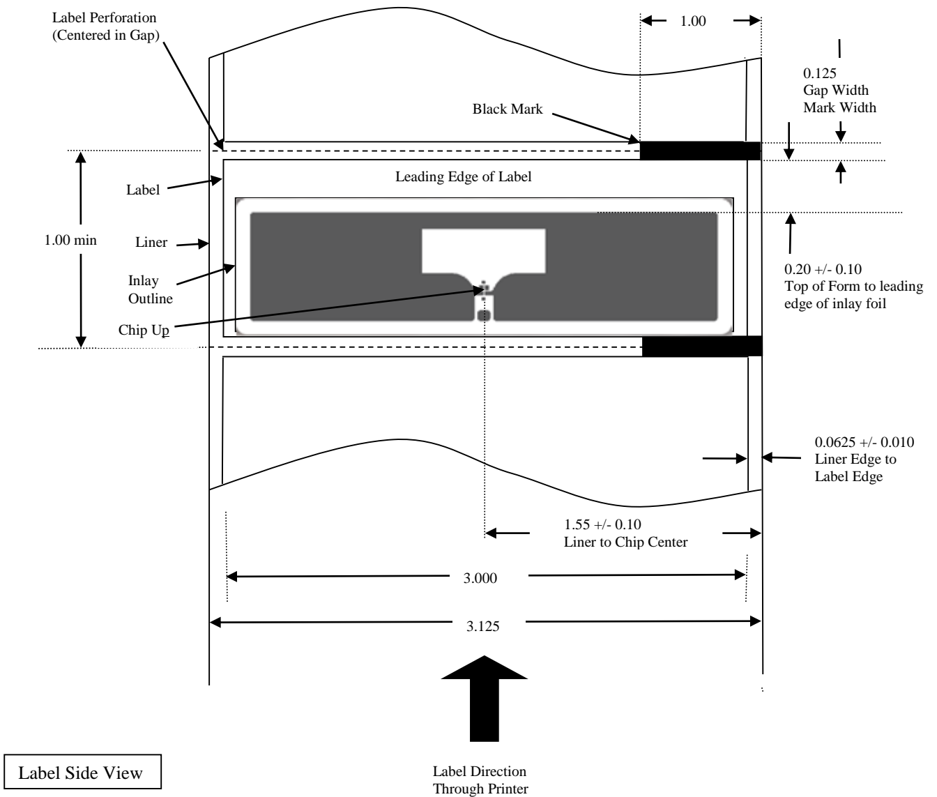
Printronix Auto ID RFID Label Requirements for SL4M “Short Pitch” Tageos EOS 400 U7 Inlay
