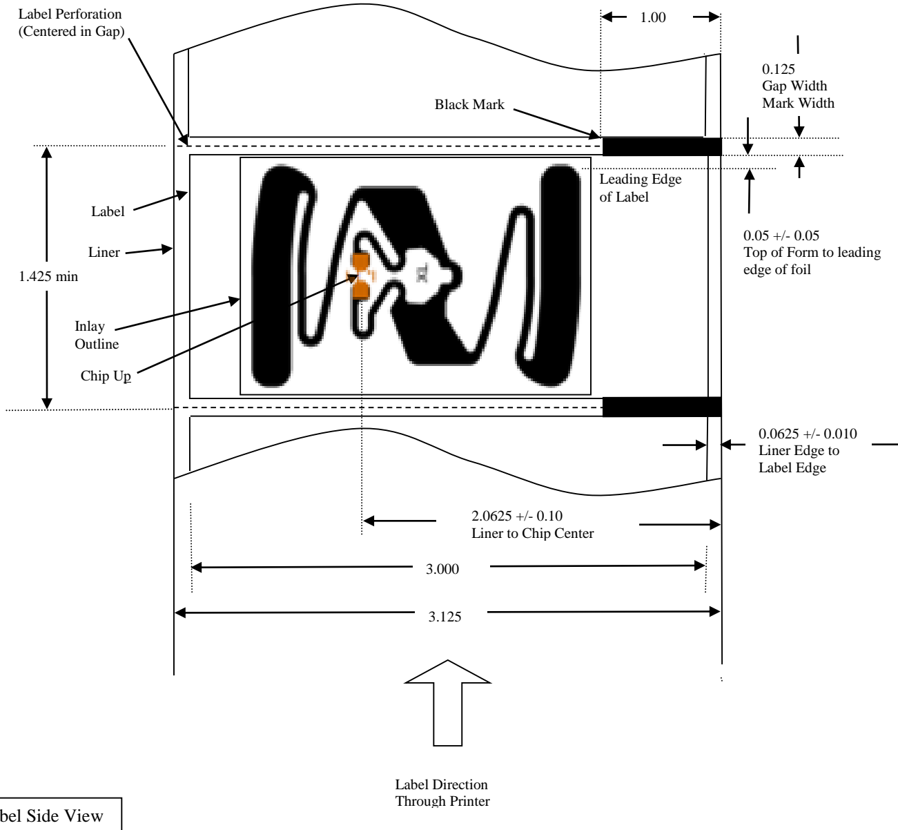
Printronix Auto ID RFID Label Requirements for SL4M “Short Pitch” Avery AD-826 Inlay
