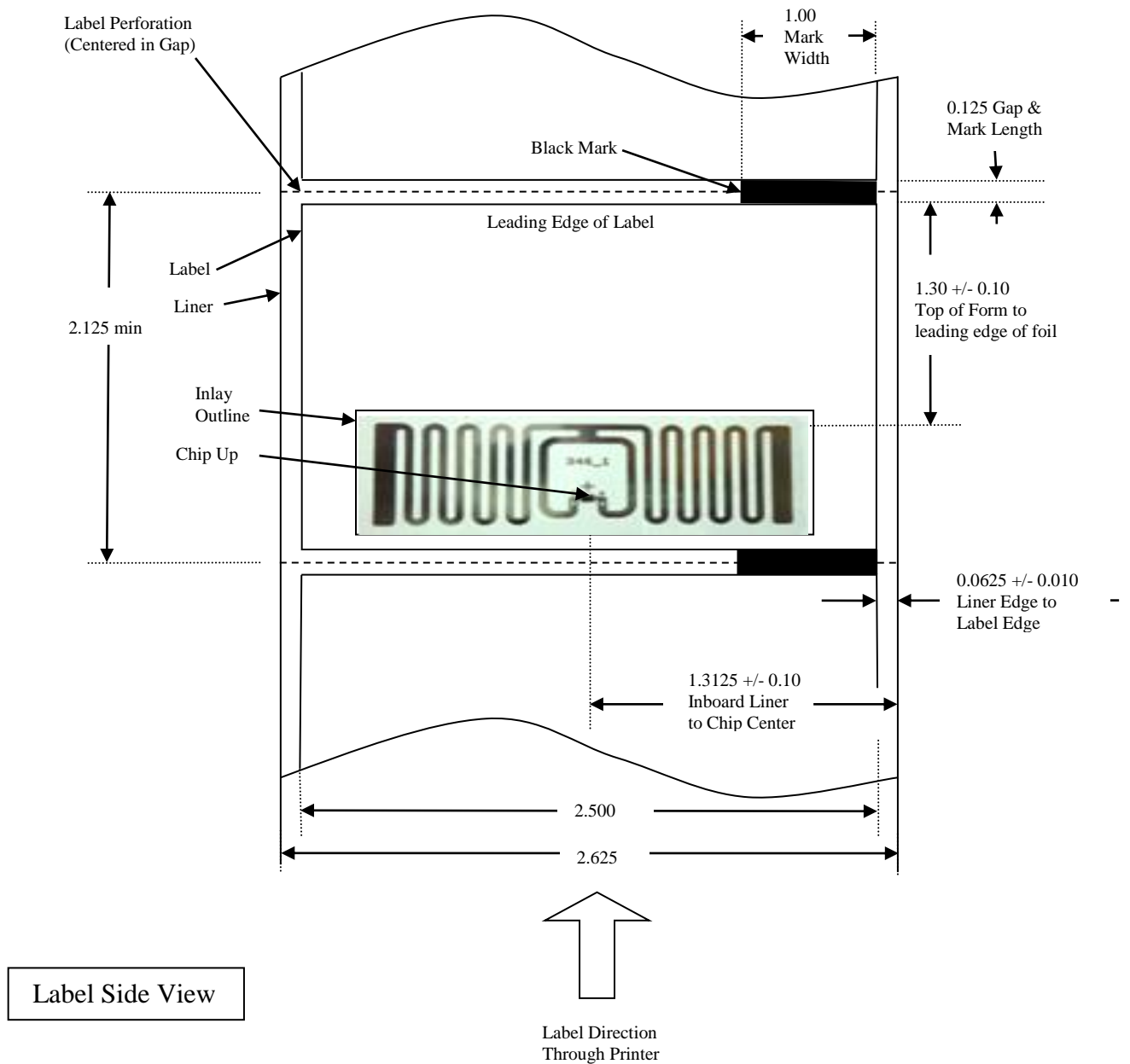
Printronix Auto ID RFID Label Requirements for SL4M/SL5r MP2 "Standard Pitch" Gen 2 Smartrac Web Lite Inlay
