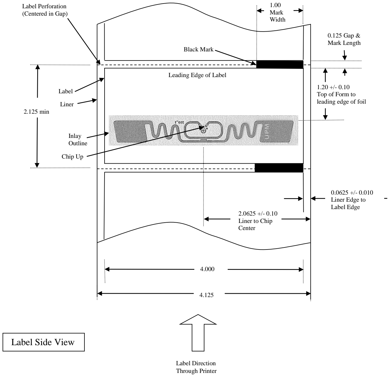
Printronic Auto ID RFID Label Requirements for MP2 Gen 2 UPM 2043 Short Inlay
