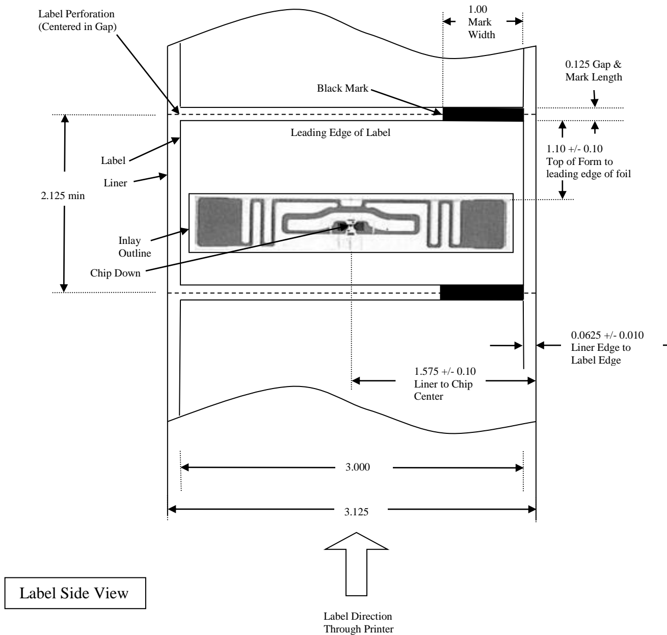
Printronix Auto ID RFID Label Requirements for SL4M/SL5r MP2 "Standard Pitch" Gen 2 Avery AD-232 Inlay
