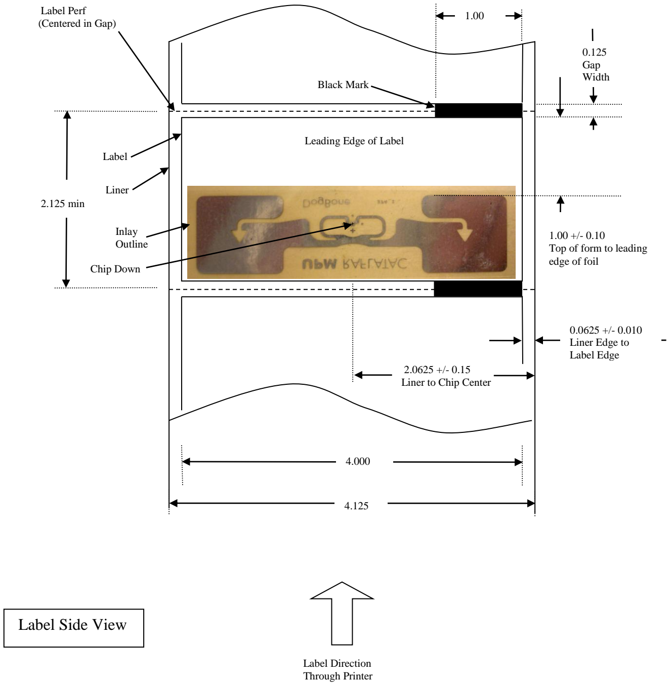
Printronic Auto ID RFID Label Requirements for MP2 Gen 2 Raflatac DogBone Ver 4 Inlay
