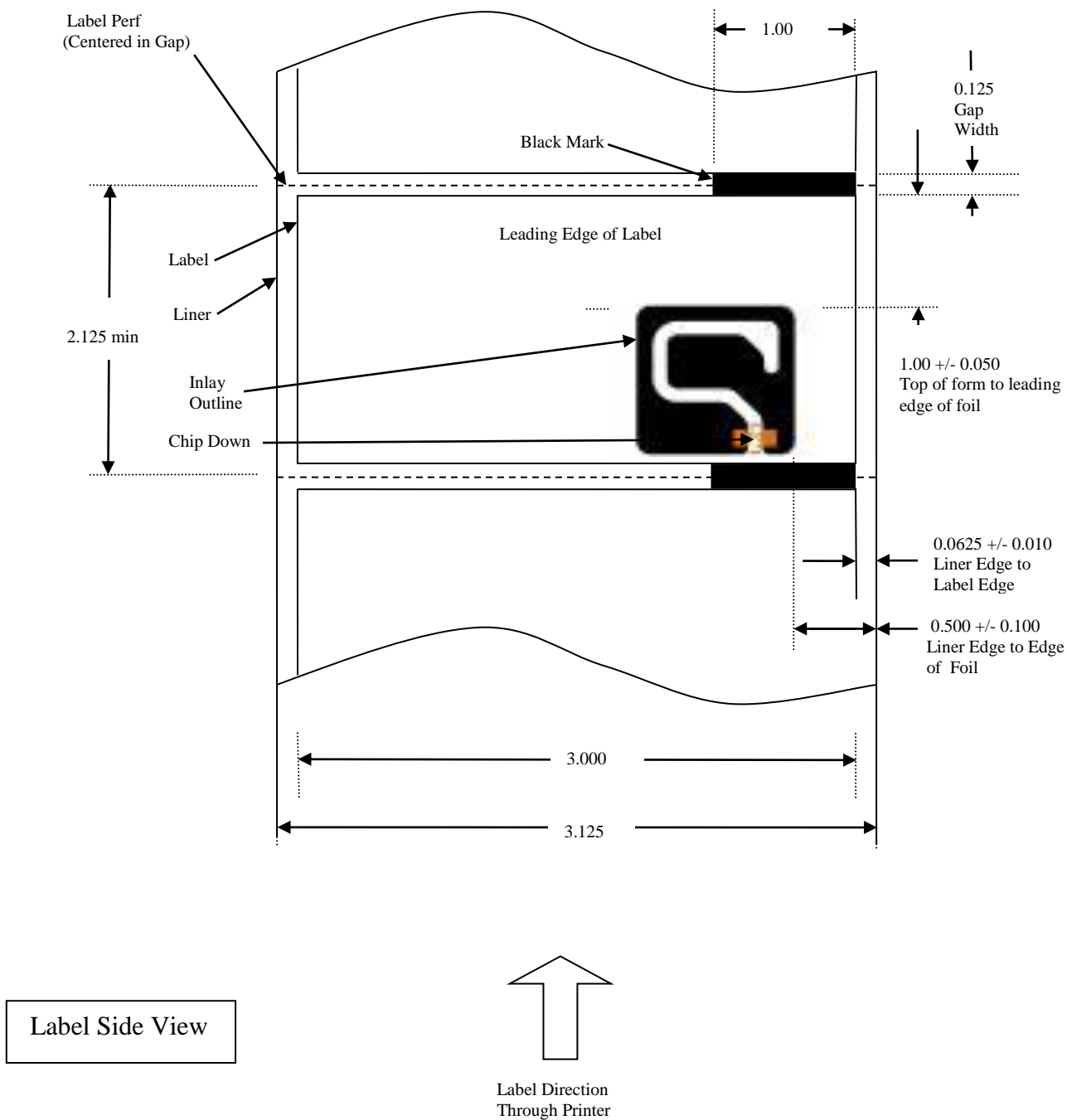
Printronic Auto ID RFID Label Requirements for MP2 Gen 2 Avery AD-814 Inlay
