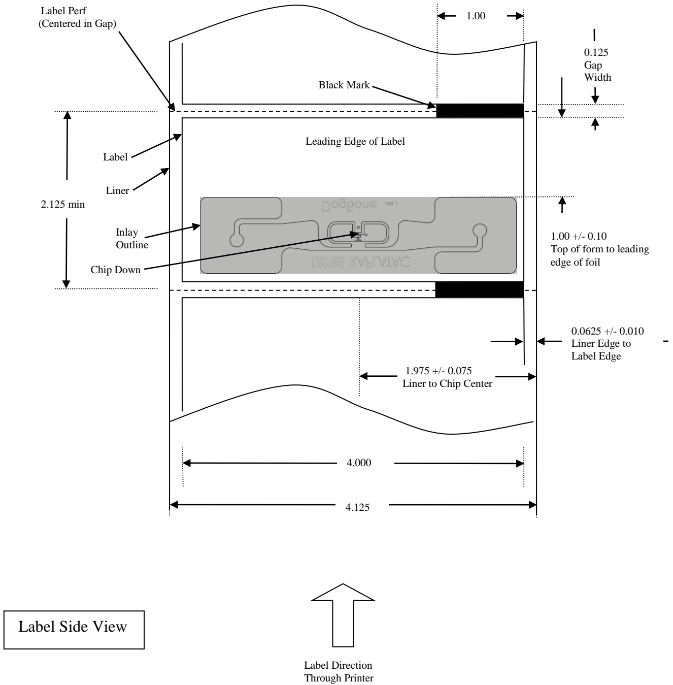
Printronic Auto ID RFID Label Requirements for MP2 Gen 2 Raflatac DogBone Ver 3 Inlay
