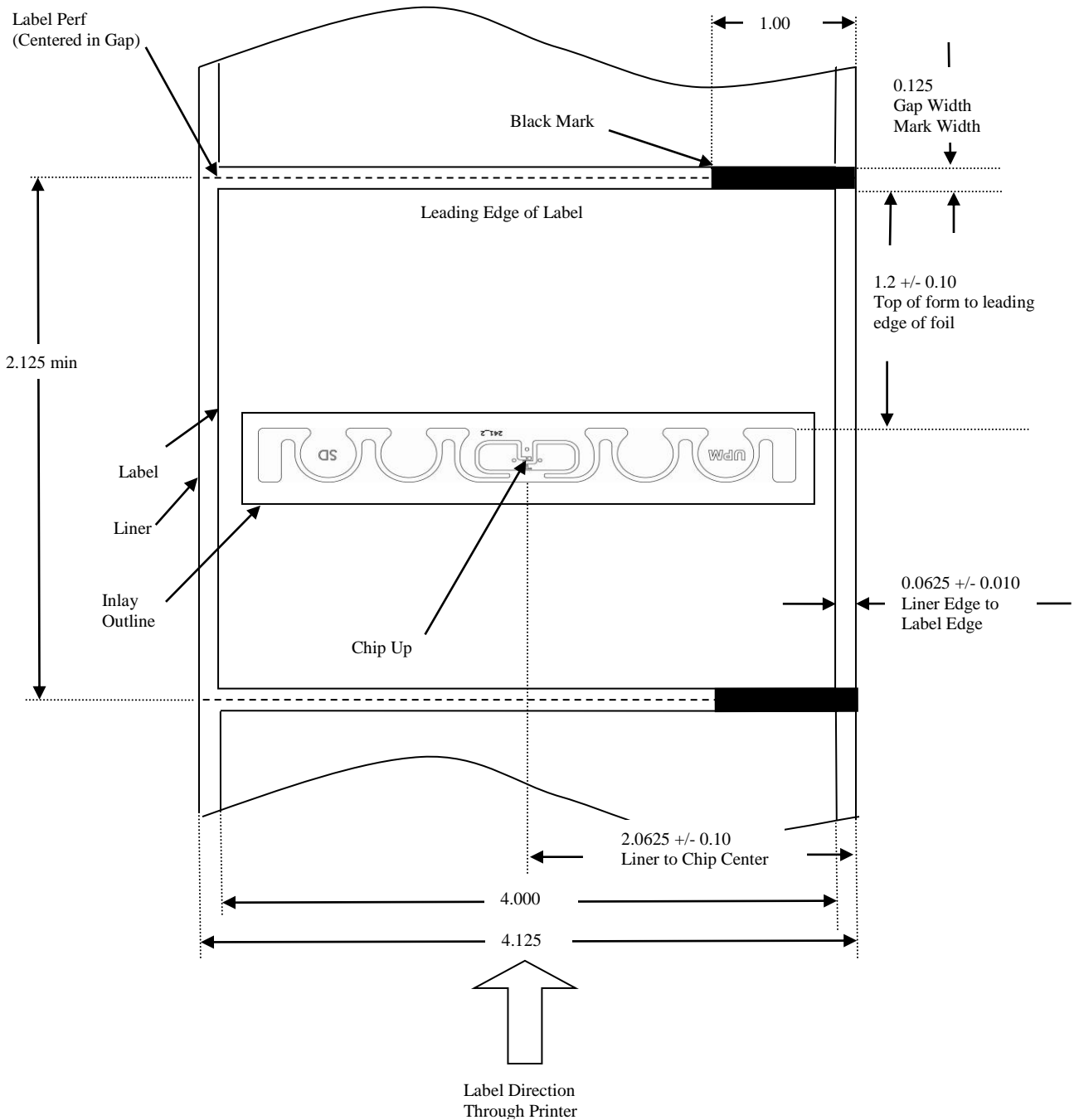
Printronic Auto ID RFID Label Requirements for MP2 UPM Raflatac Gen2 Short Dipole 3001488 Monza3 for 4in Wide x 2in Long (and Longer) Label
