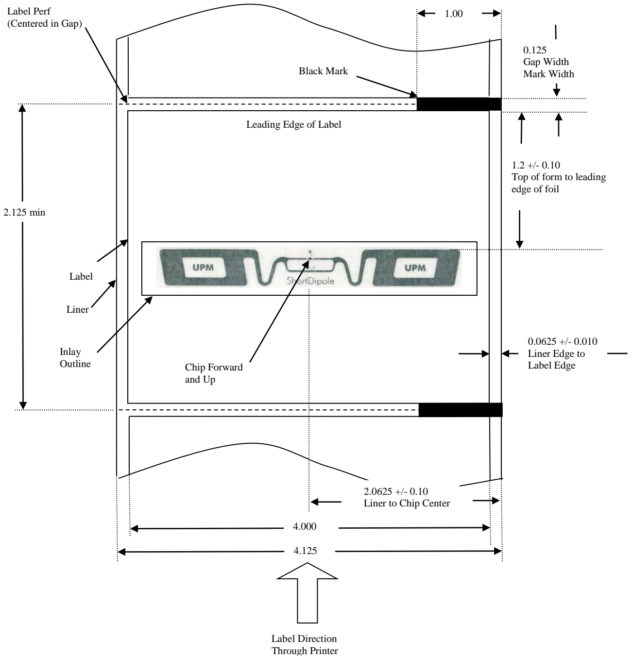
Printronic Auto ID RFID Label Requirements for MP2 UPM Raflatac Gen2 Short Dipole 3001282 Short for 4in Wide x 2in Long (and Longer) Label
